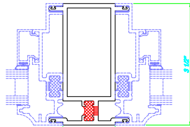
5 STRUCTURAL MULLION FOR SERIES 8300
