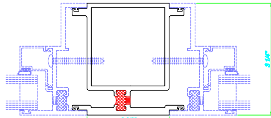
3 2 3/8" MULLION FOR SERIES 8200
