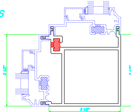
6 90° CORNER MULLION FOR SERIES 8300
