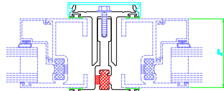
1 2" MULLION FOR SERIES 8200 / 8200
