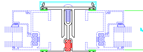
2 2 3/4" MULLION FOR SERIES 8200 / 8200
