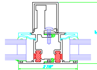
4 3" MULLION FOR SERIES 8100
