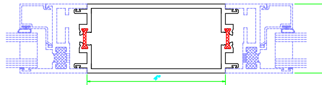
7 4" MULLION FOR SERIES 8200 / 8200
